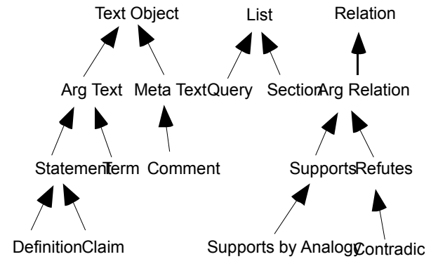
Figure 3. A typical type hierarchy. The arrows connect each type with its parent type. The top row contains the fundamental types.
